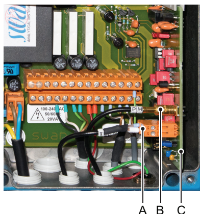
A Front end PCB B pH sensor plug C Temperature sensor plug
